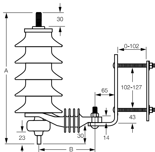
Figure 6. UltraSIL polymer-housed VariSTAR surge arrester as in Figure 4 with NEMA® crossarm hanger, see Figure 8.
