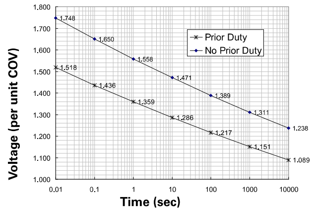
Figure 3. Temporary Overvoltage Capability (followed by U_c ), 60° C ambient, UNS and UHS. The 24 hour TOV without prior duty is 1.173 per unit of U_c .
