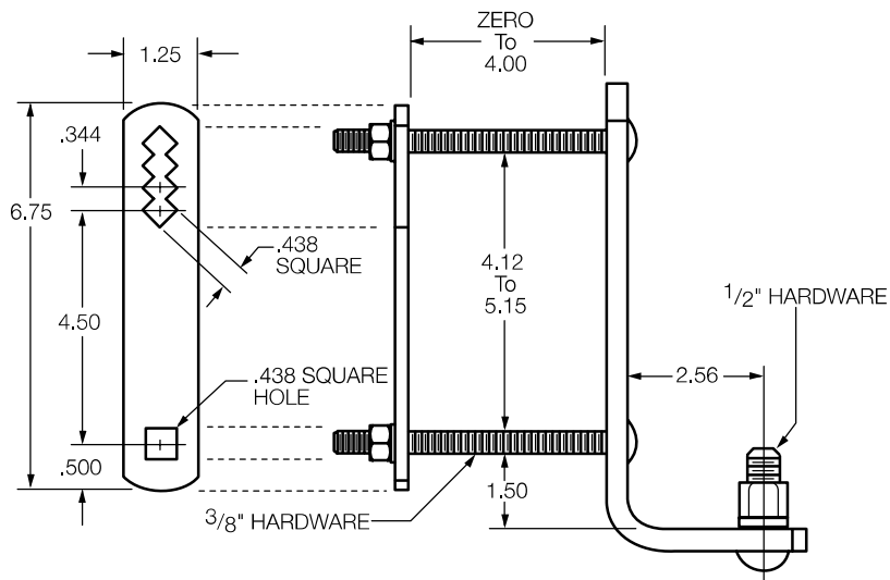
Figure 8. NEMA® crossarm hanger can be specified with a "B" in digit 13 (all dimensions are as required to be in inches, per NEMA®).
