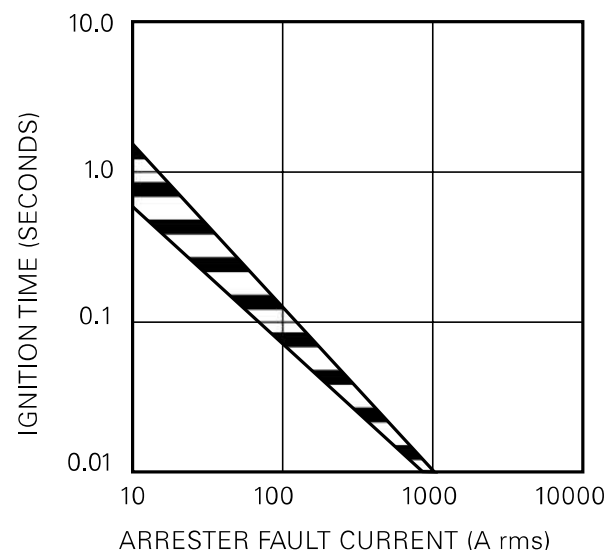
Figure 2. UNS and UHS disconnector operating characteristic.
