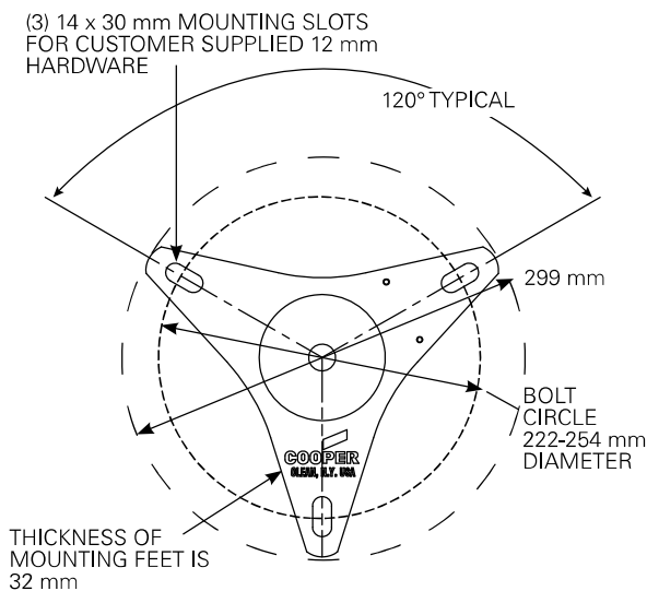
Figure 5. Base mounting.
