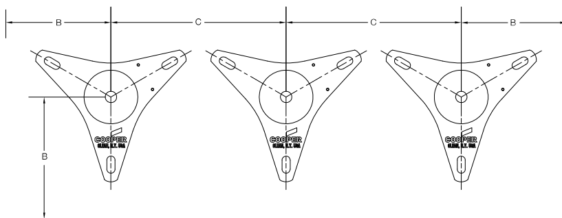
Figure 3. Three-phase in-line mounting.
