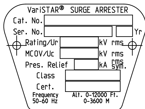
Figure 7. Detail of unit nameplate on arrester base.
