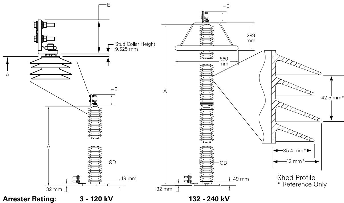
Figure 4. Outline Drawing of Standard UltraSIL Polymer-Housed VariSTAR Type U3 Surge Arresters.
